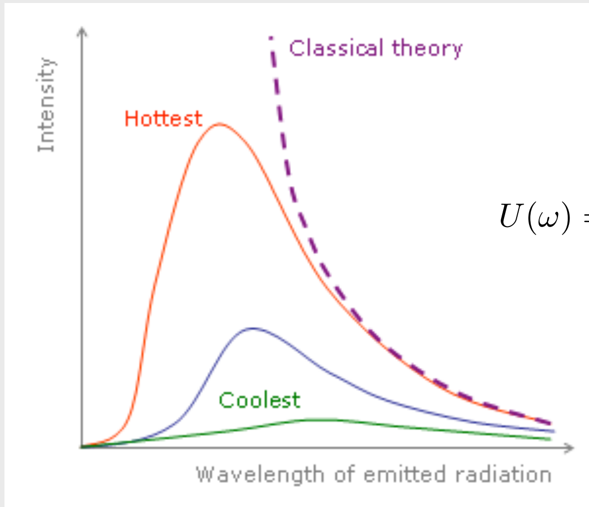
Black body spectrum
